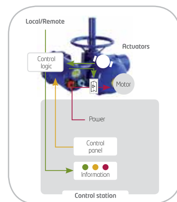
INTELLI+® control
