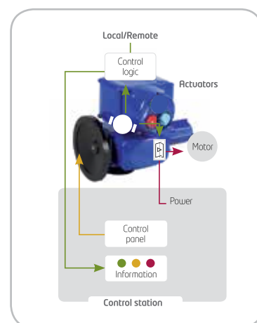
Integrated controls INTEGRAL+ / POSIGAM+
